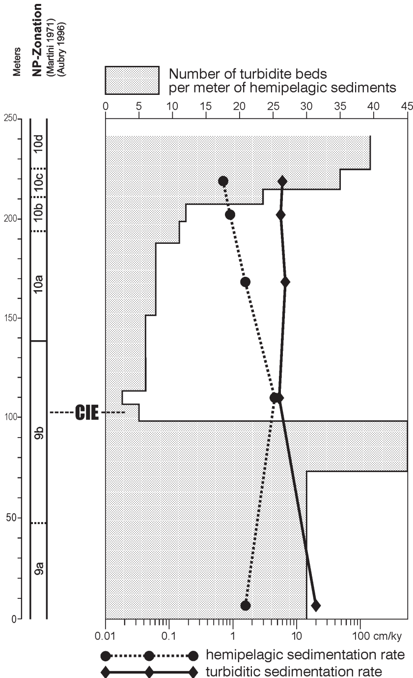
Figure 3. Relative frequency of turbidity currents and estimated turbidite and hemipelagic rates of sedimentation in nannofossil zones in the Anthering section. CIE—carbon isotope excursion,
