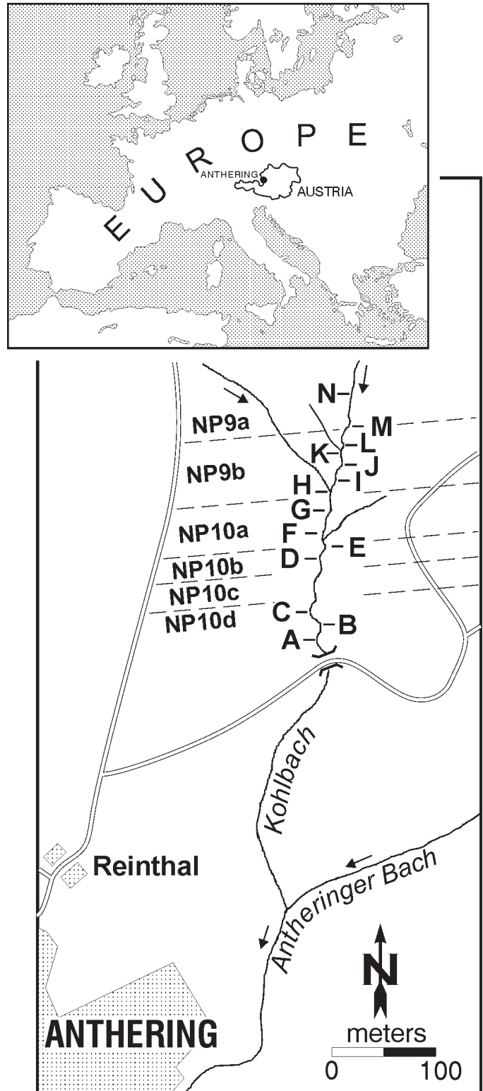
Figure 1. Position of the Anthering section, location of outcrops (A–N) and biostratigraphy of outcrops in terms of the calcareous nannoplankton standard zonation (NP Zones) of Martini (1971) and their further subdivision by Aubry (1996).
