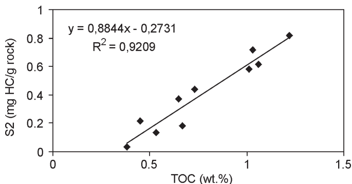
Figure 4. S2 vs. total organic carbon (TOC) diagram (Langford and Blanc-Valleron, 1990). The true average hydrogen index of samples from the Anthering Formation is 88 mgHC/gTOC.
