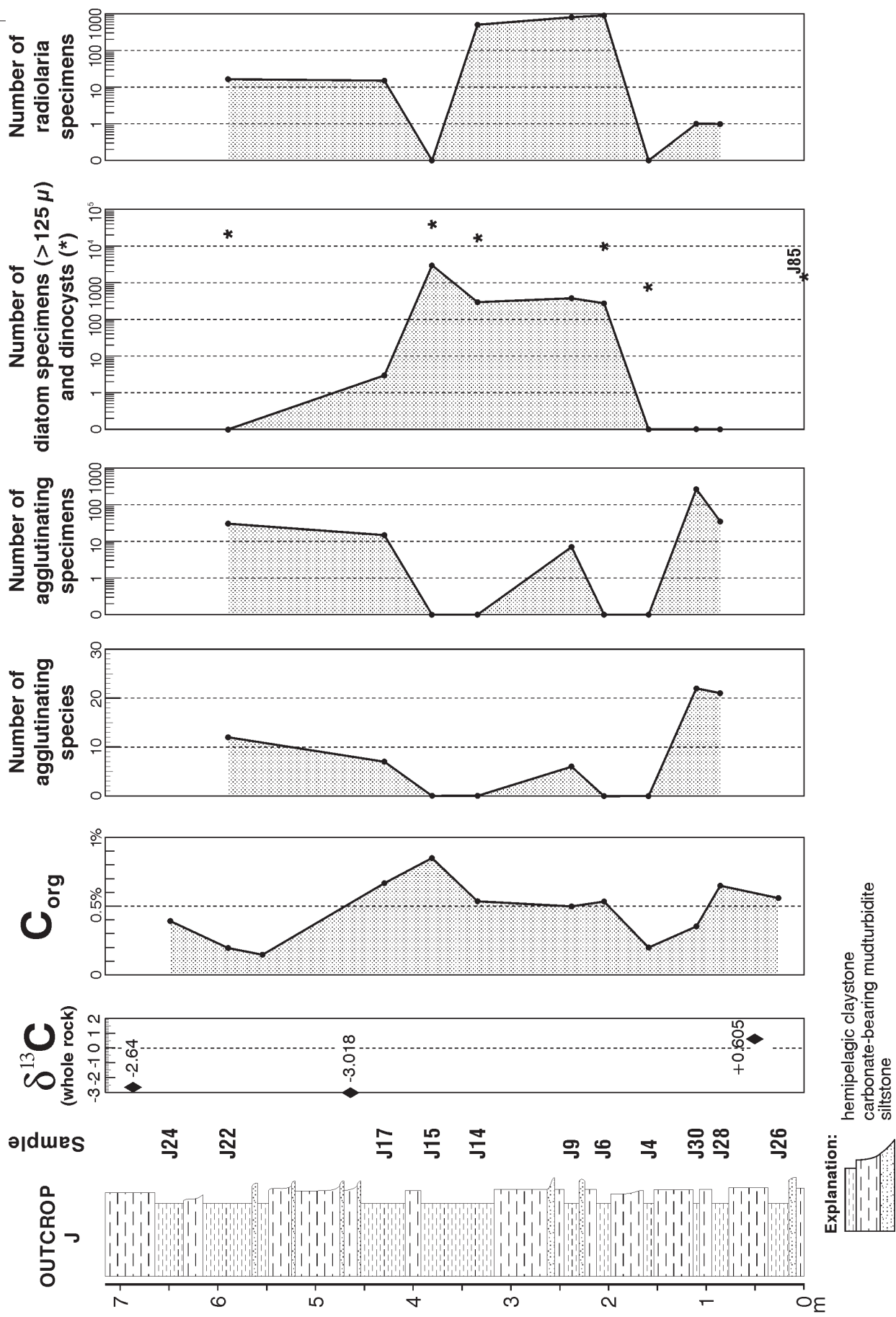
Figure 6. Detailed section of the onset of the negative carbon isotope event (CIE) displaying abundances of agglutinating foraminifera and siliceous plankton in 200 g sediment and abundances of dinoflagellates in 1 g sediment. Sample J85 was taken ~4 m below the base of the measured section.
