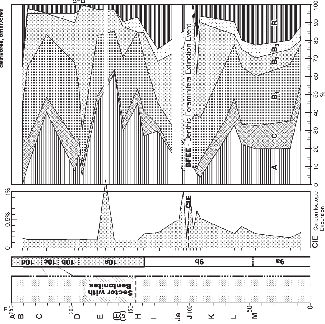
Figure 5. Distribution of organic carbon, agglutinating foraminifera and siliceous plankton within the Anthering section.
